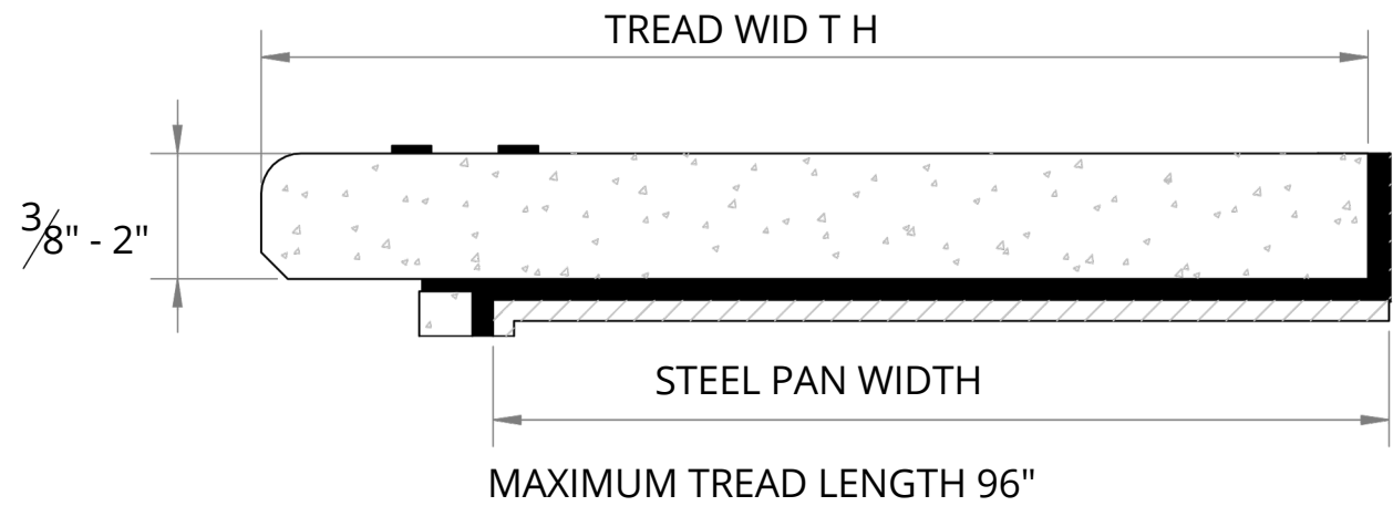
TREAD DETAIL
